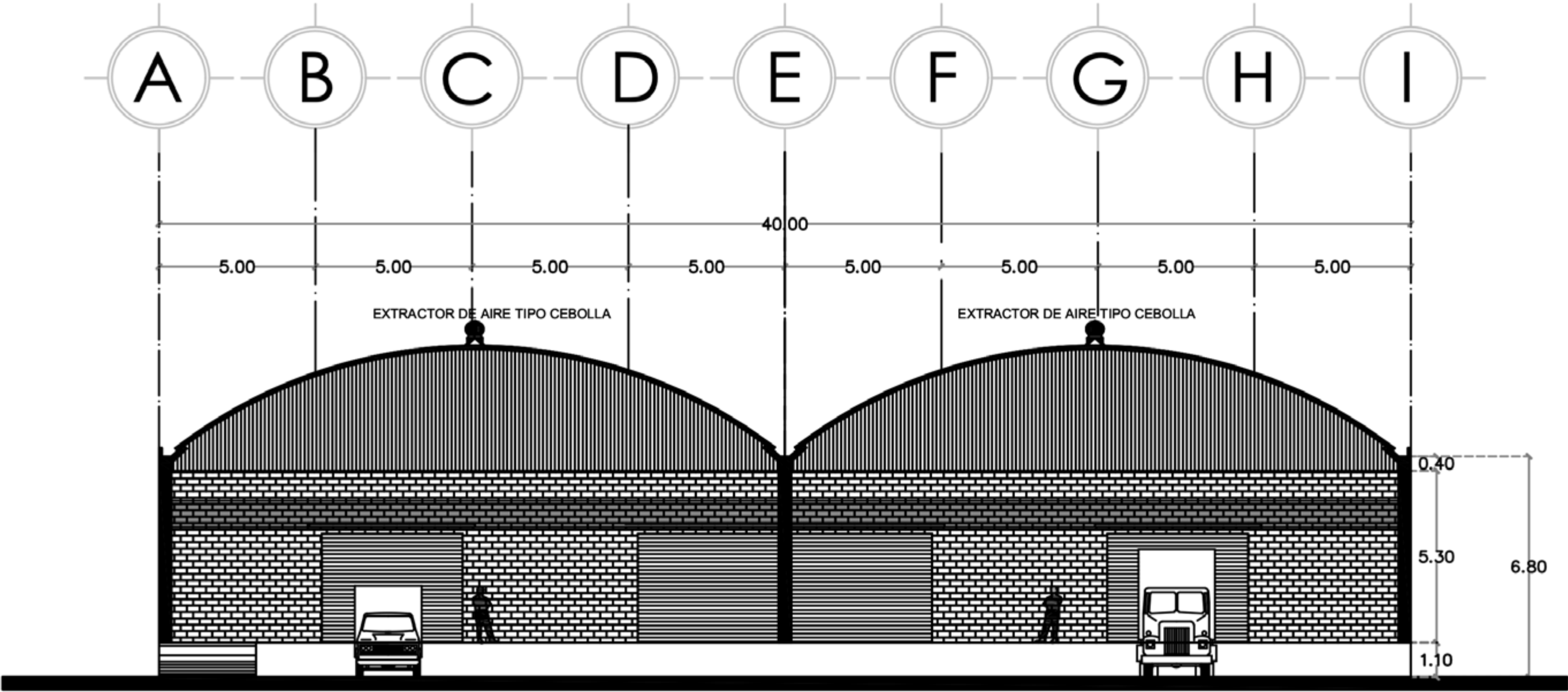
FACHADA PRINCIPAL
